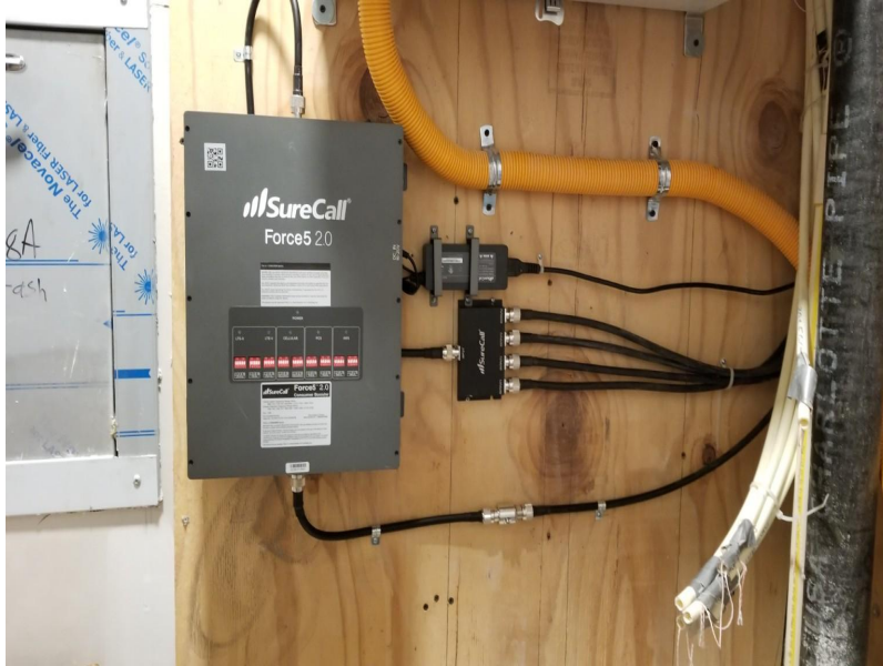
SureCall Force5 DAS Infrastructure
